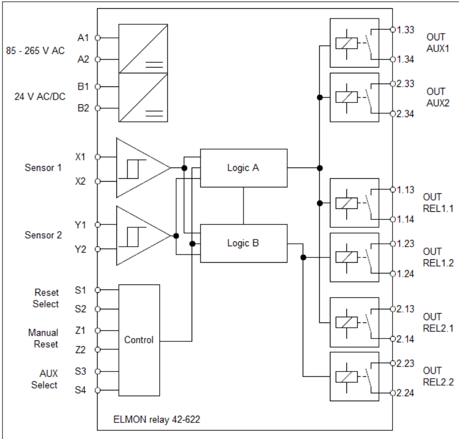
Block diagram
